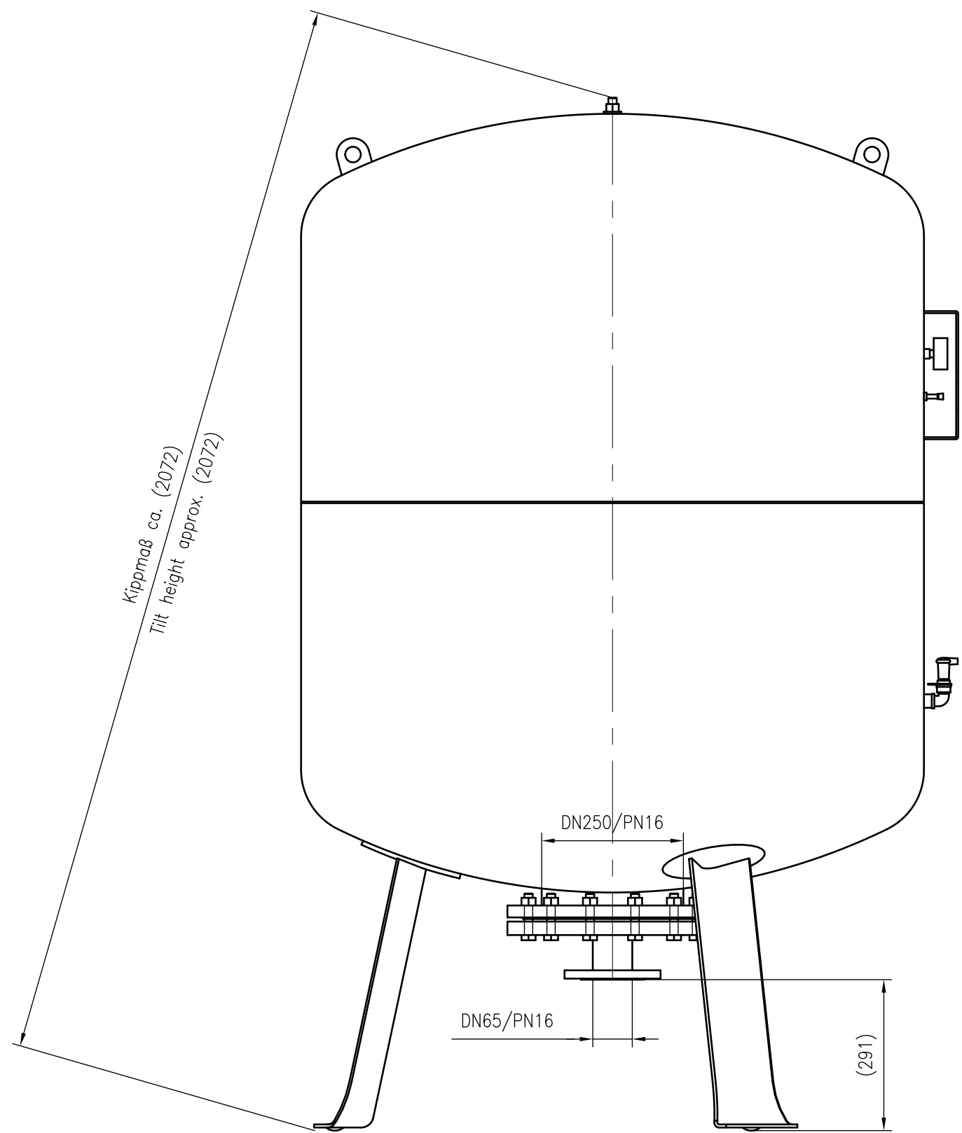
Side view
