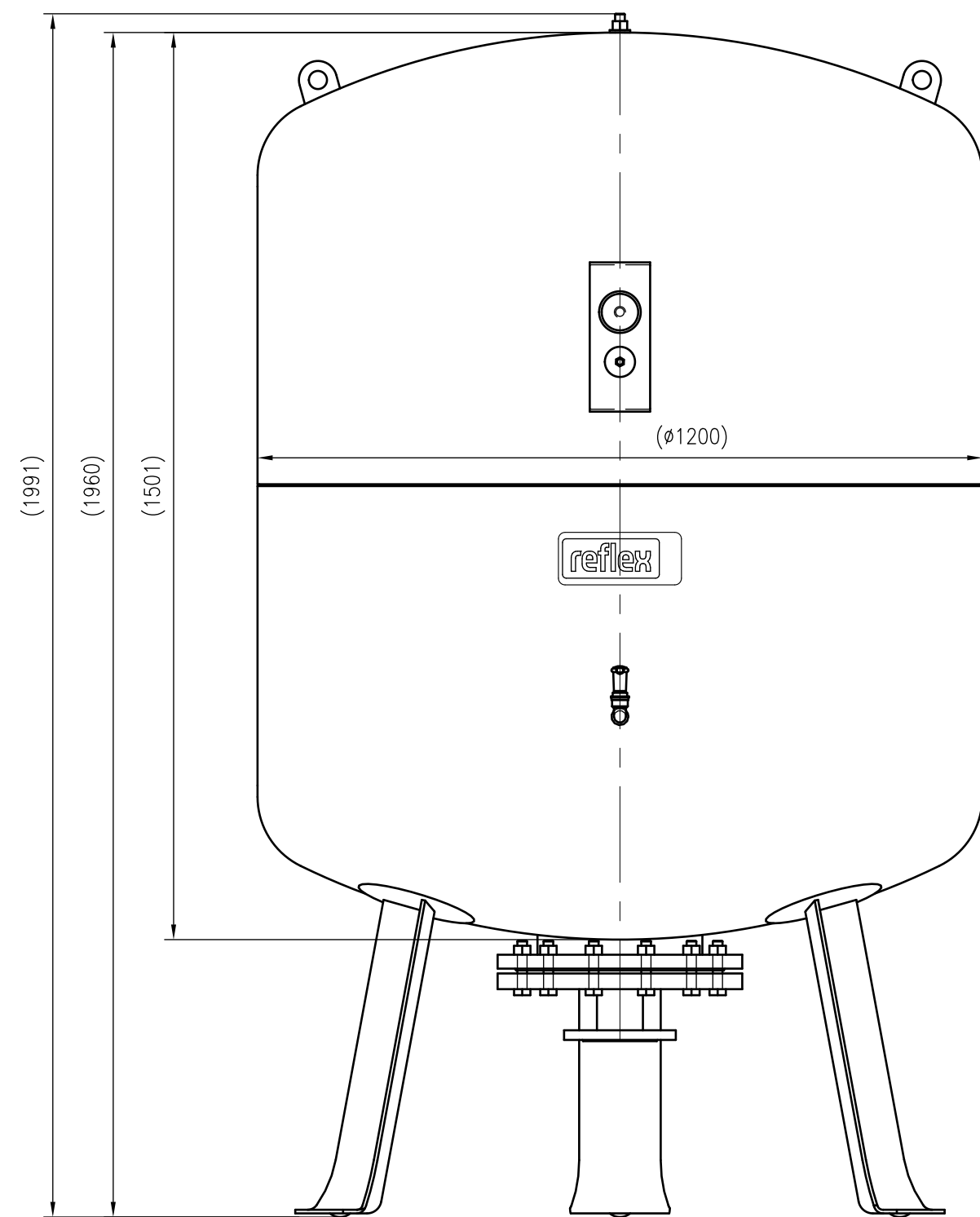
Front view
